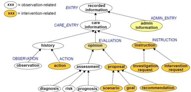
Fig. 1. The OpenEHR Ontology of Recorded Information (Beale & Heard, 2007).
