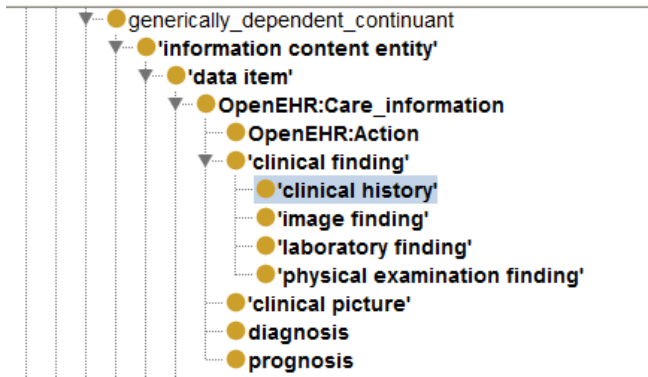
Fig. 2. The OpenEHR Care Information branch
