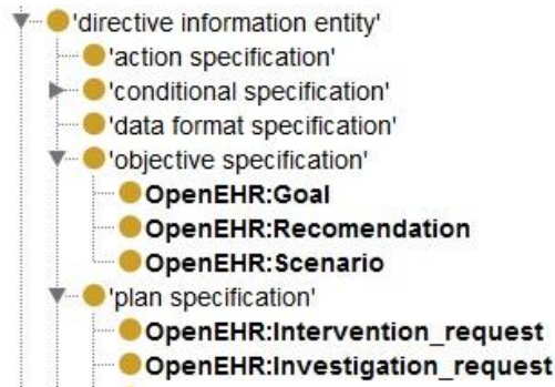
Fig. 3. The OpenEHR entry directive information branch Using this new ontology, we proceeded to analyse one archetype of each main branch (observation, action, evaluation and instruction) contained in the OpenEHR Clinical Knowledge Manager (OpenEHR Foundation, 2010). Our criteria for selection were based on published status and frequency in medical records. The findings are summarized in the next section.
